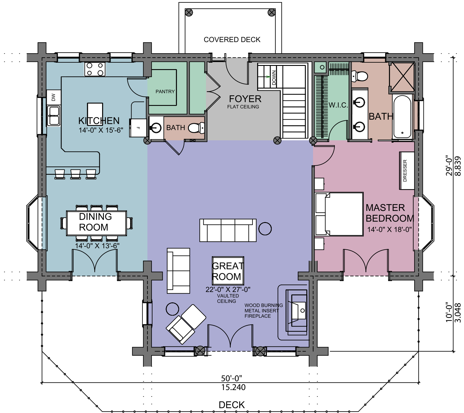
FIRST FLOOR PLAN AREA: 1633 SQ.FT. 152 SQ.M.
